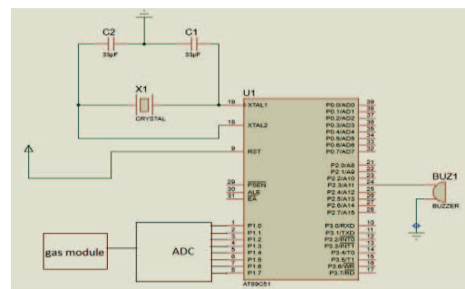
Fig. 3: Gas Leakage Detection
