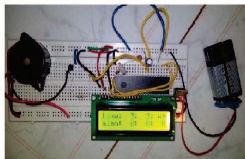
Fig. 4: Alarm fitted Digital Clock
