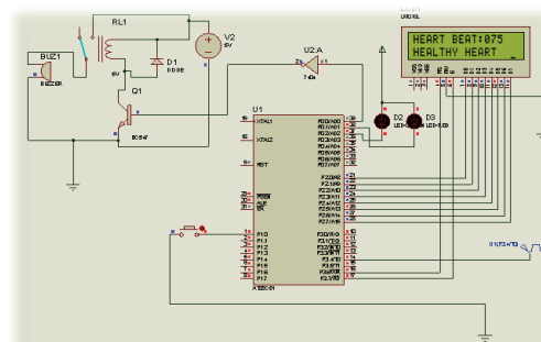
Fig. 2: Heart Beat Monitor
