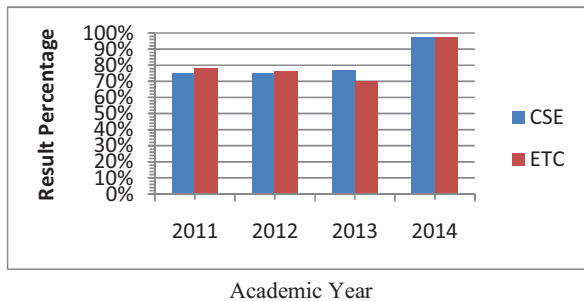
Figure 3: Result Analysis
