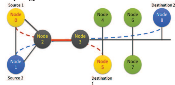
Fig 4. Network Topology
