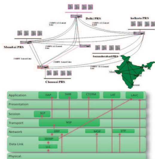
Fig 3. Network topology and Communication model and Protocols
