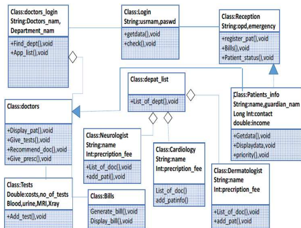
Figure 2. UML diagram for HMS.
