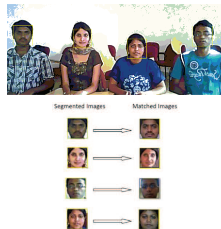
Fig. 6. Segmentation and matching of faces
