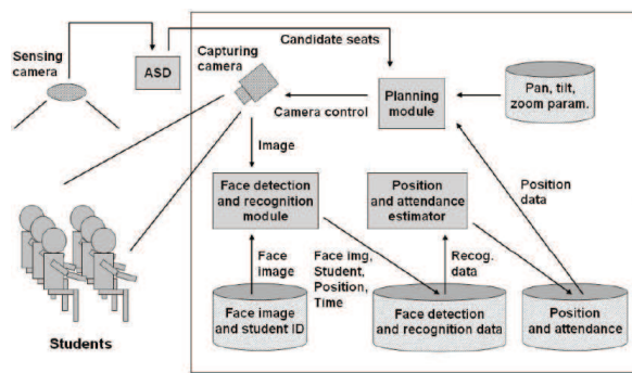
Fig. 5. Automatic attendance system
