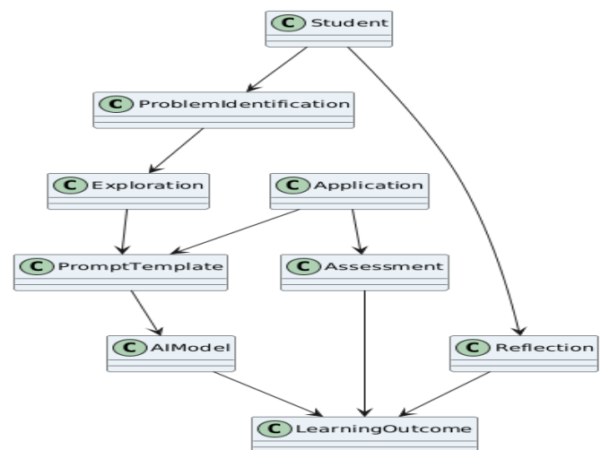
Fig. 1. PEARL UML Class Diagram
