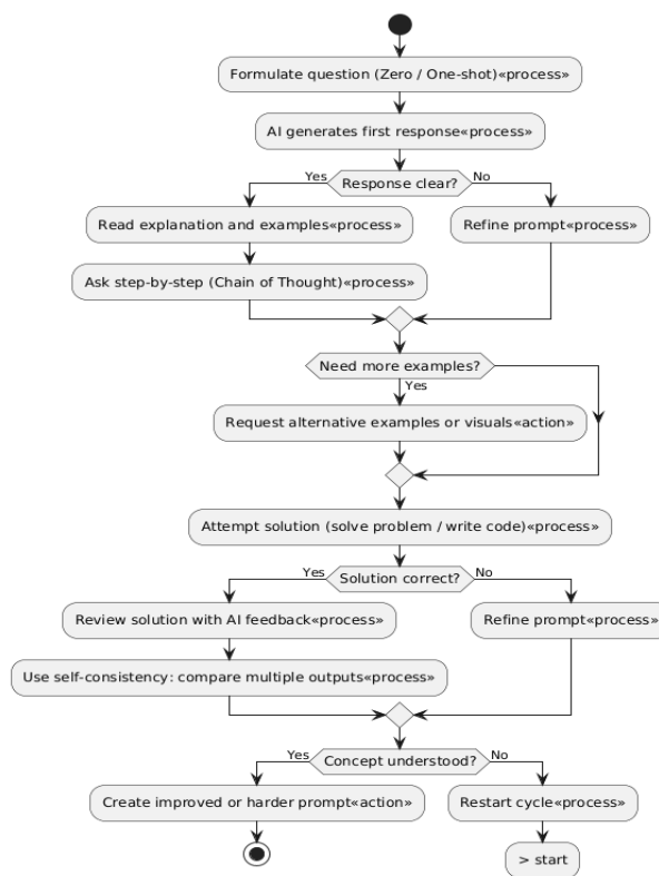
Fig. 2. PEARL Flowchart of Interactive Prompting
