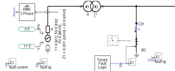
Fig. 12: PSCAD simulated network.
