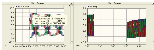
Fig.9: Graphs for Fault Current and Voltage
