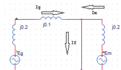
Fig.7: Equivalent circuit when fault occurs
