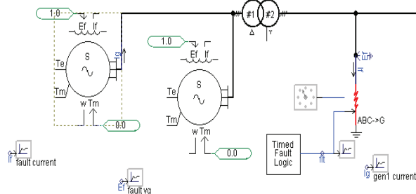
Fig. 3: Network in PSCAD
