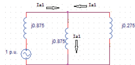
Fig.11: Interconnection of Sequence Networks
