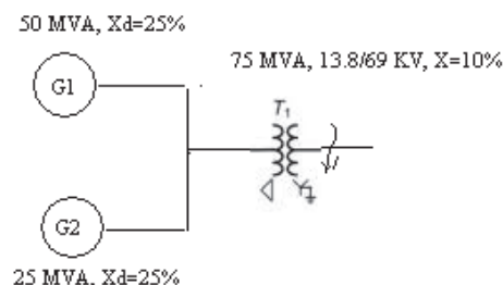
Fig.1: Single Line Diagram
