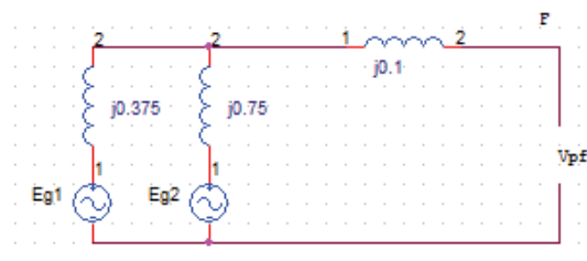
Fig 2: Equivalent reactance diagram
