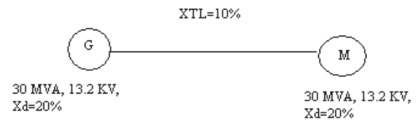
Fig. 5: Single Line Diagram
