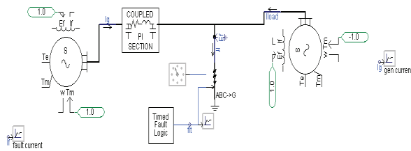
Fig.8: PSCAD network
