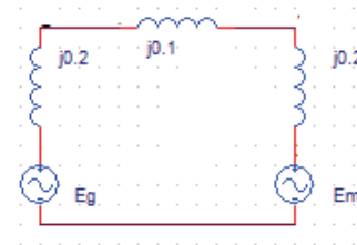
Fig. 5: Single Line Diagram
