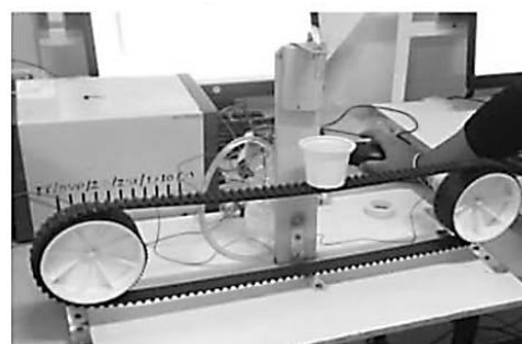
Fig.3. Bottle filling system
