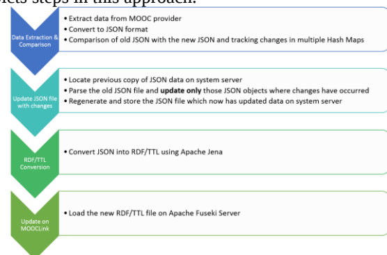
Figure 5: Incremental Update approach
