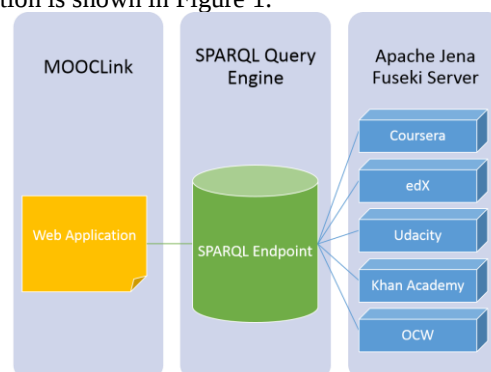
Figure 1: MOOCLink - High-level Architecture
