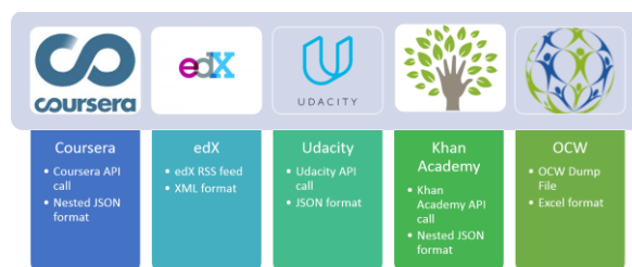
Figure 2: Data Sources for MOOCLink
