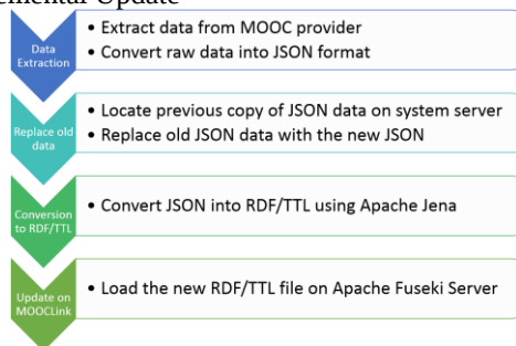
Figure 4: Naive Batch Update Approach
