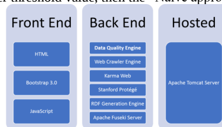
Figure 8: MOOCLink - System Design
