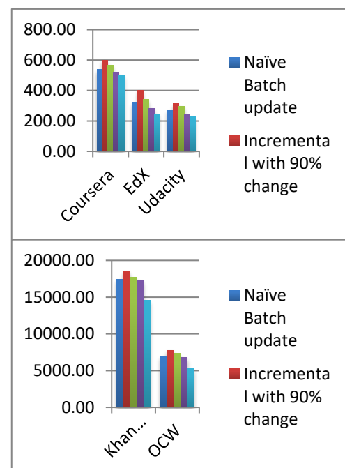
Figure 10: Results of Incremental update approach
