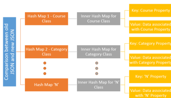
Figure 6: JSON comparison in Incremental Update approach
