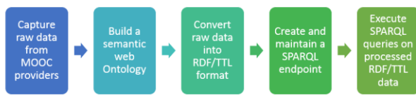
Figure 3: Linked Data Generation Process
