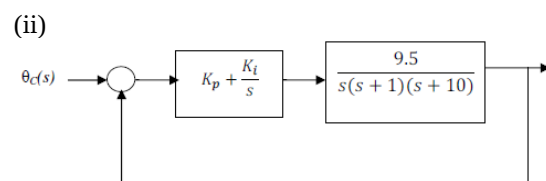
Fig. 8 Reduced block diagram
