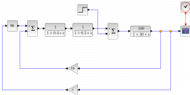
Fig. 2 X – COS model of AGC
