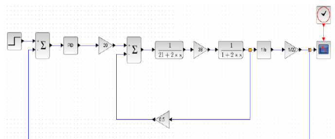
Fig. 7 SCILAB model of robot arm
