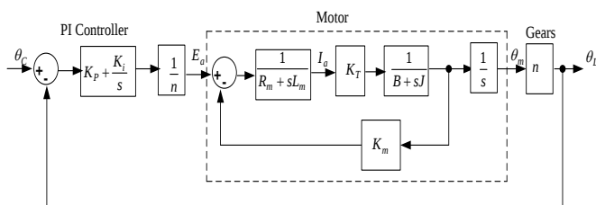
Fig. 6 Model of a servo controlled joint of a robot arm
