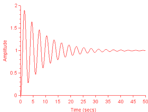
Fig. 8 System response with PI – Controller
