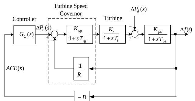
Fig. 1 Automatic Generation Control Model
