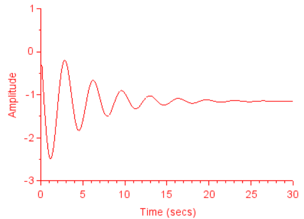
Fig. 3 System response with P – Controller
