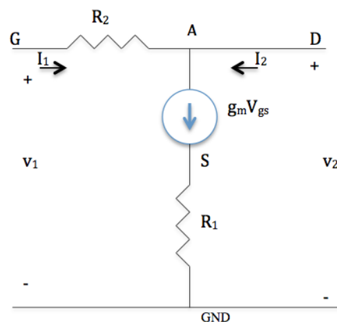
Fig. 9 Model of BB Amplifier
