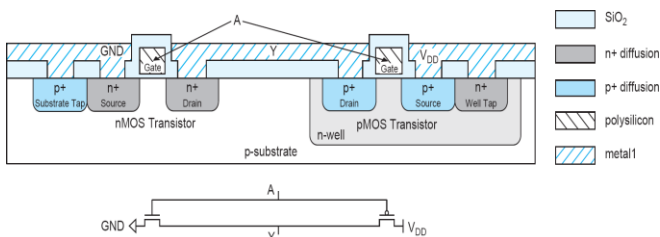
Fig . 4 CMOS Inverter
