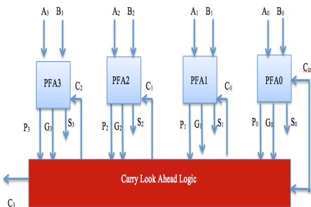
Figure 6 Carry Look Ahead Adder
