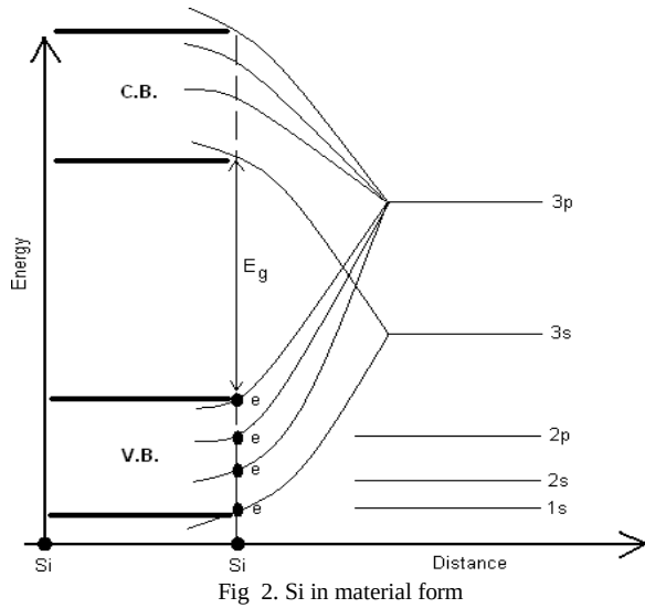
Fig 2. Si in material form
