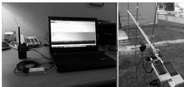
Figure 7 - (a) Packet Radio Communication, Handheld Radio and Antenna (Portable Radio Communication)
