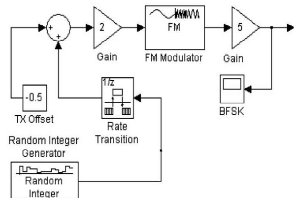
Fig. 5. Implementation of BFSK using simulink tool
