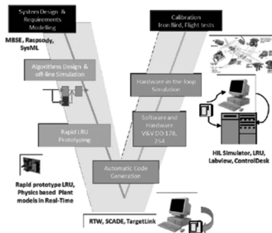
Fig.1: MBD work flow within V cycle
