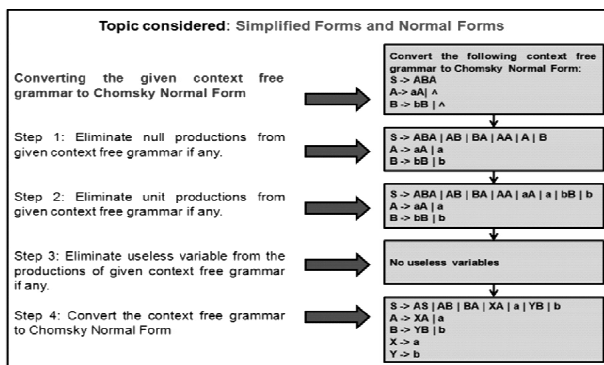
Fig. 3: Conversion of context free grammar to Chomsky Normal form
