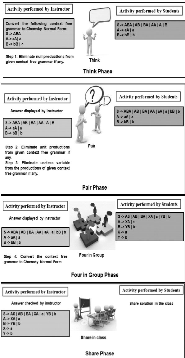
Fig. 6: T24S for converting CFG to CNF
