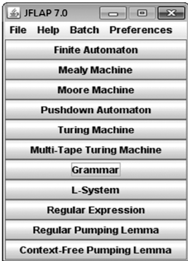
Fig. 10: JFLAP 7.0
